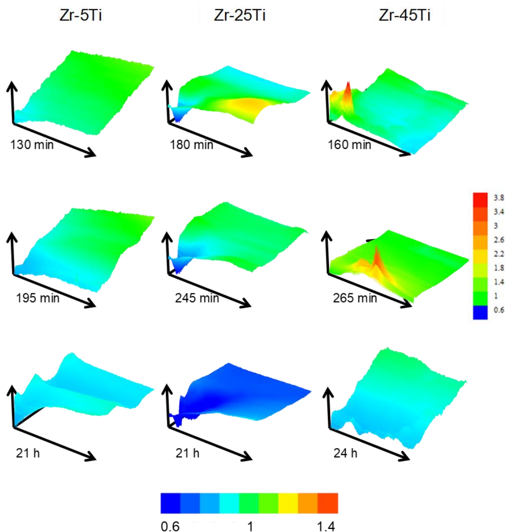
Figure 5. Representative feedback mode 2-D scans of 500 \times 500 \mu\text{m}^2 dimension on oxidized binary Zr-Ti alloys immersed in acidified Ringer's solution at 37^\circ\text{C} . Images in a column were obtained over the same sample and area, indicated at the top of the figure. Time immersion is given below each scan. The color scale gives the normalized current in all scans except for the scan measured on Zr-45Ti after 265 min, which is plotted with its own color scale.
