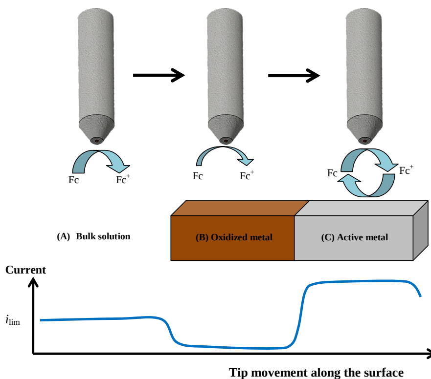
Figure 3. Limiting electrochemical responses for the tip current depending on the surface condition of the Zr-Ti alloys exposed to Ringer’s solution during amperometric SECM operation using ferrocene-methanol (Fc) as redox mediator. (A) Current attains a diffusion-controlled limiting current value in bulk solution; (B) Negative feedback occurs over the oxide-covered surface, which blocks the diffusion pathways for Fc; (C) Positive feedback happens over conductive alloy surfaces that are able to regenerate ferrocene-methanol by reducing the ferrocenium ion (Fc + ) formed at the tip.
