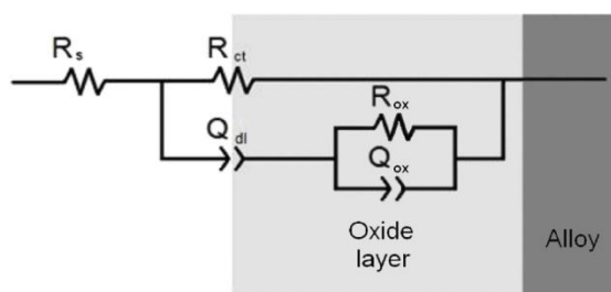
Figure 2. Equivalent electric circuit employed to fit the experimental EIS spectra.
