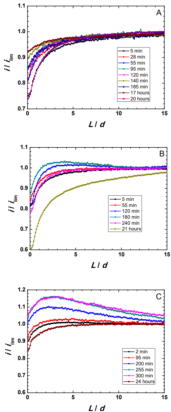
Figure 4. Feedback mode Z-approach curves on oxidized binary Zr-Ti alloys immersed in acidified Ringer's solution at 37 °C. (A) Zr-5Ti; (B) Zr-25Ti; (C) Zr-45Ti.
