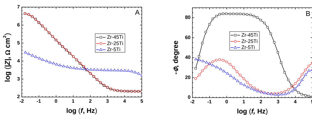
Figure 1. Bode plots acquired by EIS on binary Zr-Ti alloys (oxidized in air at 500 ^{\circ}\text{C} for 4 h) after 1-day immersion in PBS at 37 ^{\circ}\text{C} . (A) Bode-amplitude, and (B) Bode-phase diagrams.
