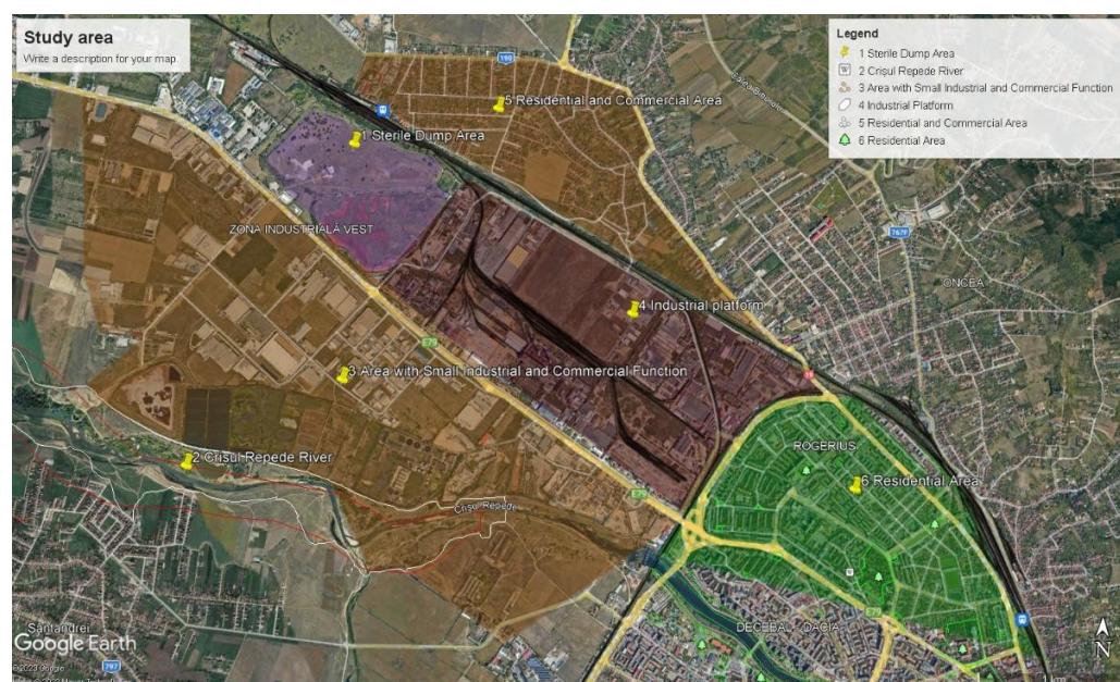
Figure 1. Research area and location of the red sludge dump.
