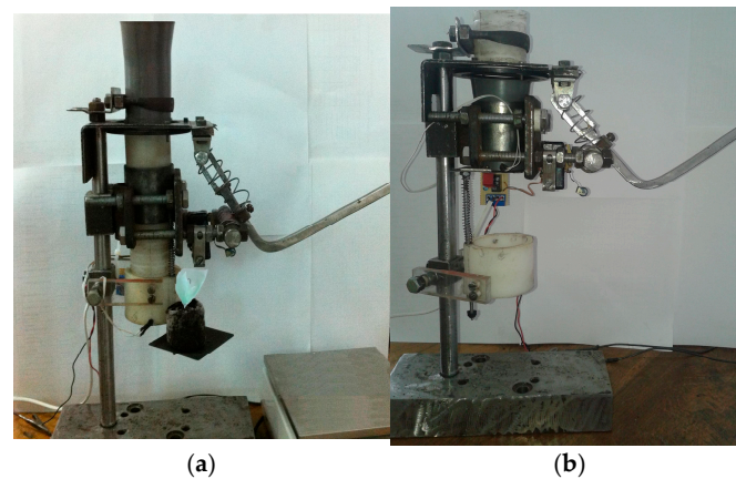
Figure A3. Auxiliary installation for gravity transport simulation. (a) Height adjustment for Transport II; (b) height adjustment for Transport III.
