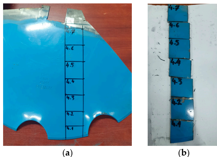
Figure 1. Extraction and preparation of radial samples. (a) Radial marking and segmentation of the disc surface before sectioning; (b) extracted radial samples.
