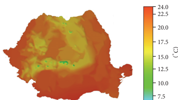
FIGURE 10: The map of the estimated temperatures for July, for the year 2030, obtained using the model ET30.
