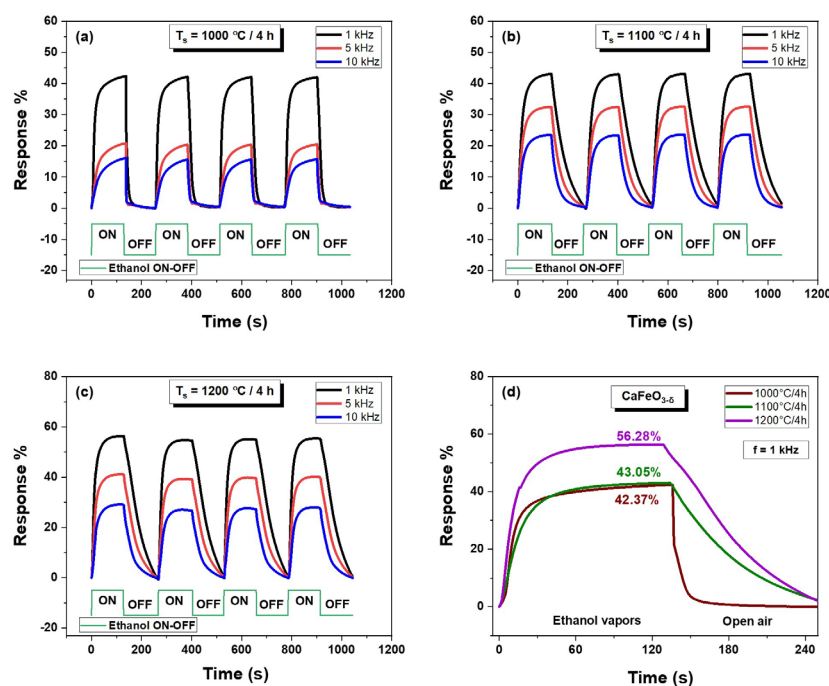
Figure 11. (a–c) Gas sensitivity responses of \text{CaFeO}_{3-\delta} ceramics sintered at different temperatures (ethanol/air atmosphere at room temperature cycle for 4 cycles) and (d) comparison of the impedance response of all samples during one exposure cycle.
