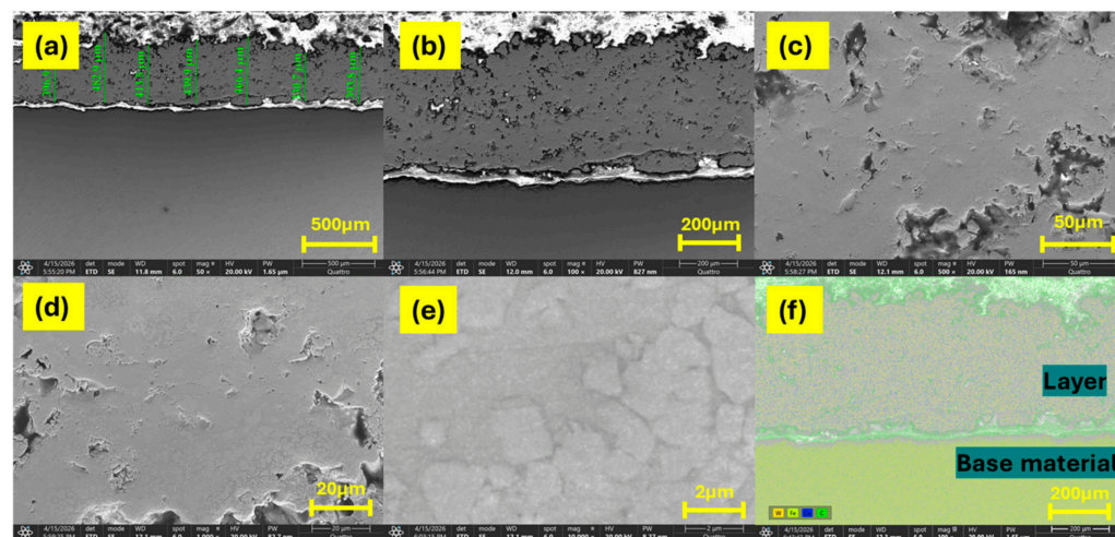
Figure 11. Cross-sectional SEM images of the WOKA 3101 coating on the mainshare at (a) 50×, (b) 100×, (c) 500×, (d) 1000×, (e) 10,000× and (f) EDS mapping.
