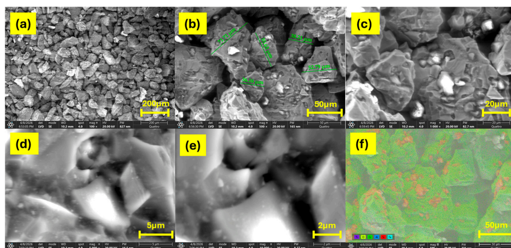
Figure 5. SEM images of Metco 136CP powder ( \text{Cr}_2\text{O}_3 - \text{SiO}_2 - \text{TiO}_2 ): (a) 100 \times (b) 500 \times (c) 1000 \times (d) 5000 \times ; (e) 10,000 \times (f) EDS mapping.
