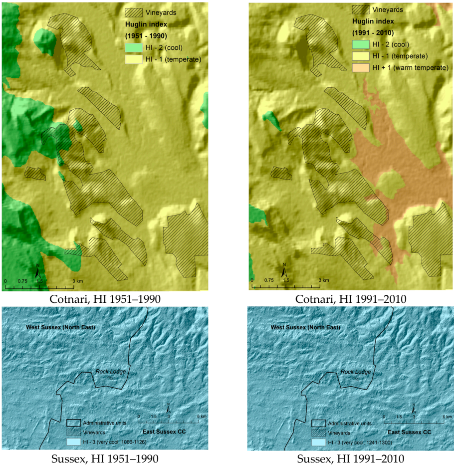
Figure 2. Shifts in the spatial distribution of the Huglin Index (HI) for the 1951–1990 and 1991–2010 time periods in studied wine regions.
