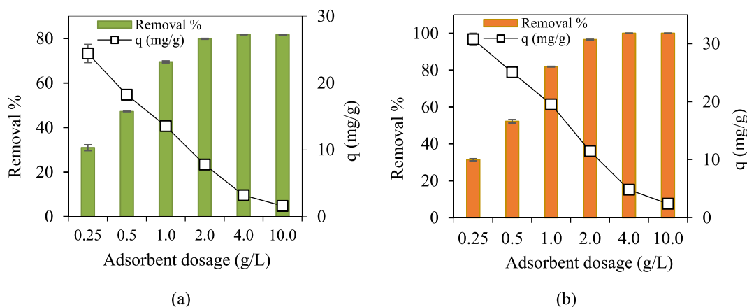
Fig. 7. Removal effectiveness and adsorbed amount by (a) RA and (b) EA, at various biosorbent concentrations, C_0 = 20 mg/L Pb(II), pH 5 \pm 0.5 , T = 23 \pm 1 °C, 4 h reaction time.
