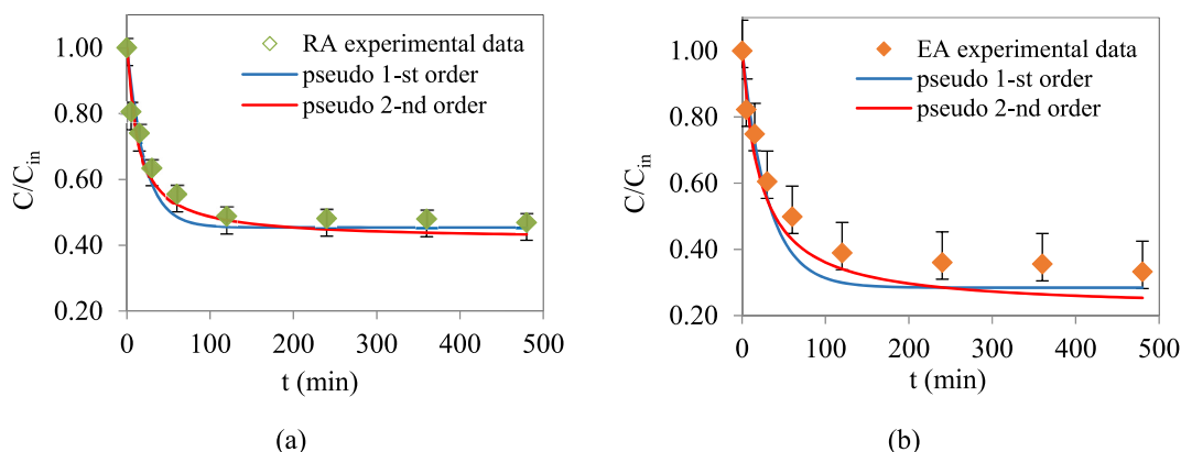
Fig. 8. Kinetics for Pb (II) biosorption on (a) RA and (b) EA at C_0 = 20 mg/L Pb(II), C_s = 0.5 g/L biosorbent dosage, T = 23 \pm 1 °C: experimental points and pseudo-first (1st) and pseudo-second (2nd) order model.
