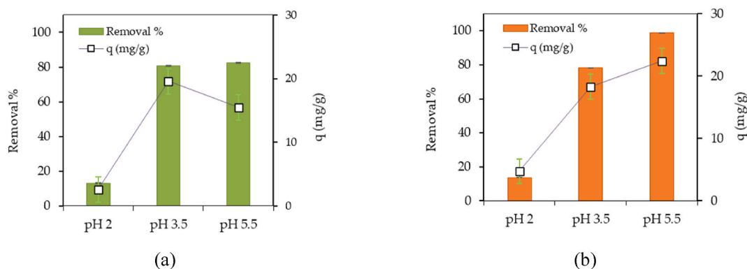
Fig. 6. pH effect on lead adsorption, C_0 = 20 mg/L Pb(II), T = 23 \pm 1 °C, 4 h contact time, C_s = 0.5 g/L (a) RA and (b) EA.
