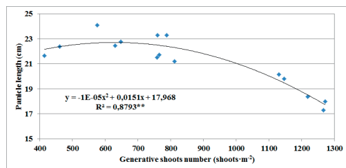
Figure 1. Correlation between generative shoots number and panicle length
