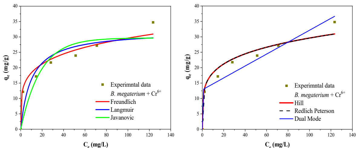
Figure 8. Graphical representation of adsorption isotherms applied to experimental data of \text{Cr}^{6+} biosorption by Bacillus megaterium inactive biomass.
