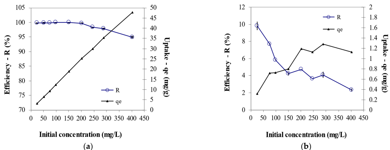
Figure 5. Effect of initial metal concentration on biosorption efficiency and metal uptake capacity of (a) Cr^{6+} and (b) total chromium by Rhodotorula sp. inactive biomass (pH = 1, contact time = 48 ore, biosorbent dosage = 8 g/L, temperature = 25 °C).
