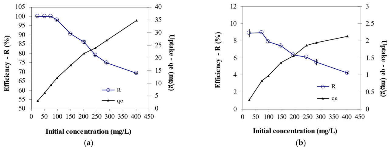
Figure 4. Effect of initial metal concentration on biosorption efficiency and metal uptake capacity of (a) Cr^{6+} and (b) total chromium by B. megaterium inactive biomass (pH = 1, contact time = 48 ore, biosorbent dosage = 8 g/L, temperature = 25 °C).
