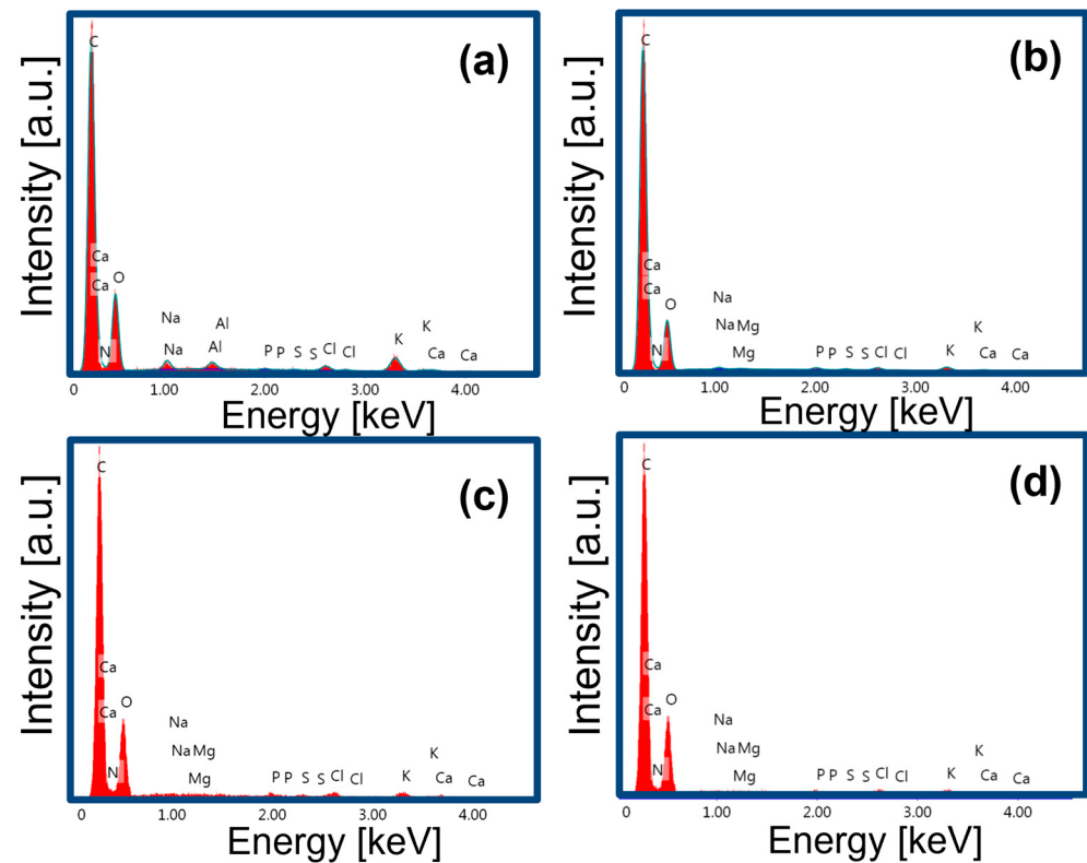
Figure 3. SEM-EDX spectrum of PPP (a), control whey cheese (RCC) (b), PPP-supplemented cheese: RCP6 (c) and RCP6 (d).
