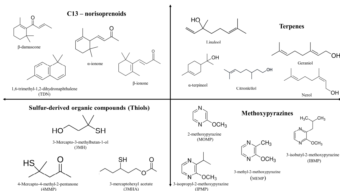
Figure 3. Chemical structure representation of the key aromatic compounds present in grapes.
