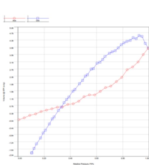
Fig. 1. The adsorption /desorption isotherm and the pore-size distribution curves for diminazene aceturate/ \beta -cyclodextrin
