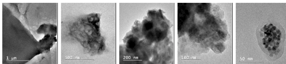
Fig.9. TEM images for the complex DIMA- \alpha -CD
