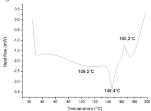
Fig.4. DSC analysis of diminazene aceturate/ \beta -cyclodextrin complex
