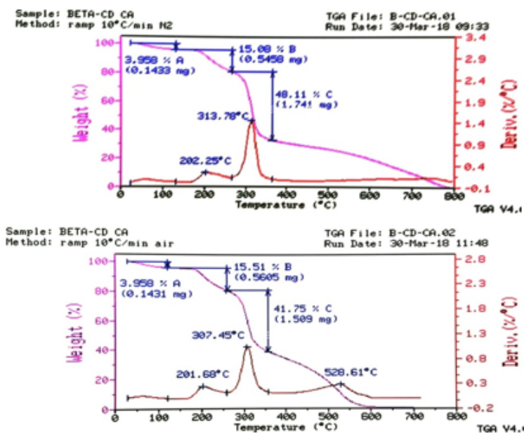
Fig.3. Termogravimetric analysis in inert gas and in synthetic air for diminazene aceturate/ \beta -cyclodextrincomplex
