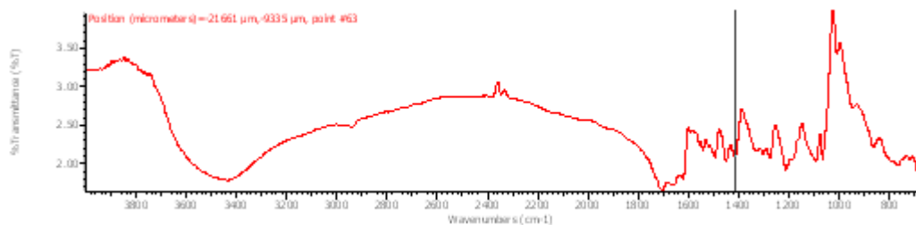
Fig.7. FTIR images of the complex DIMA- \alpha -CD surface
