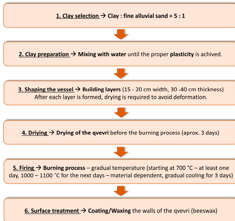
Figure 3. Steps for manufacturing qvevri vessels.
